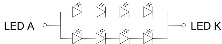
LED CIRCUIT
